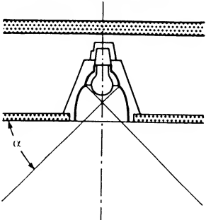
⑩ Shading angle ( = 30^\circ/40^\circ/50^\circ )
